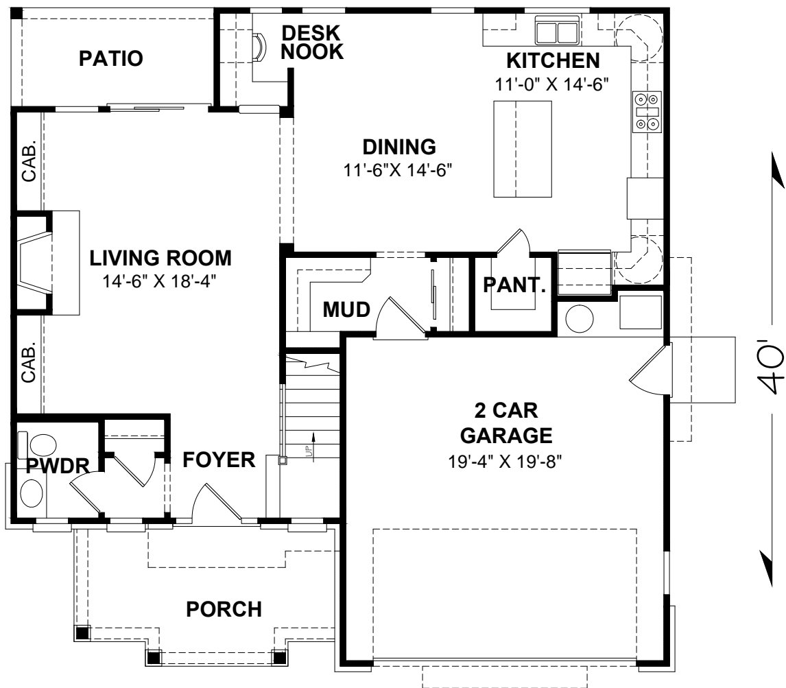
40' MAIN FLOOR PLAN
